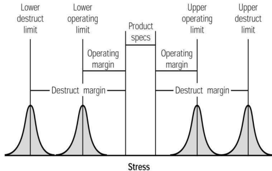
Figure 4. Operating & Destruct Limits
